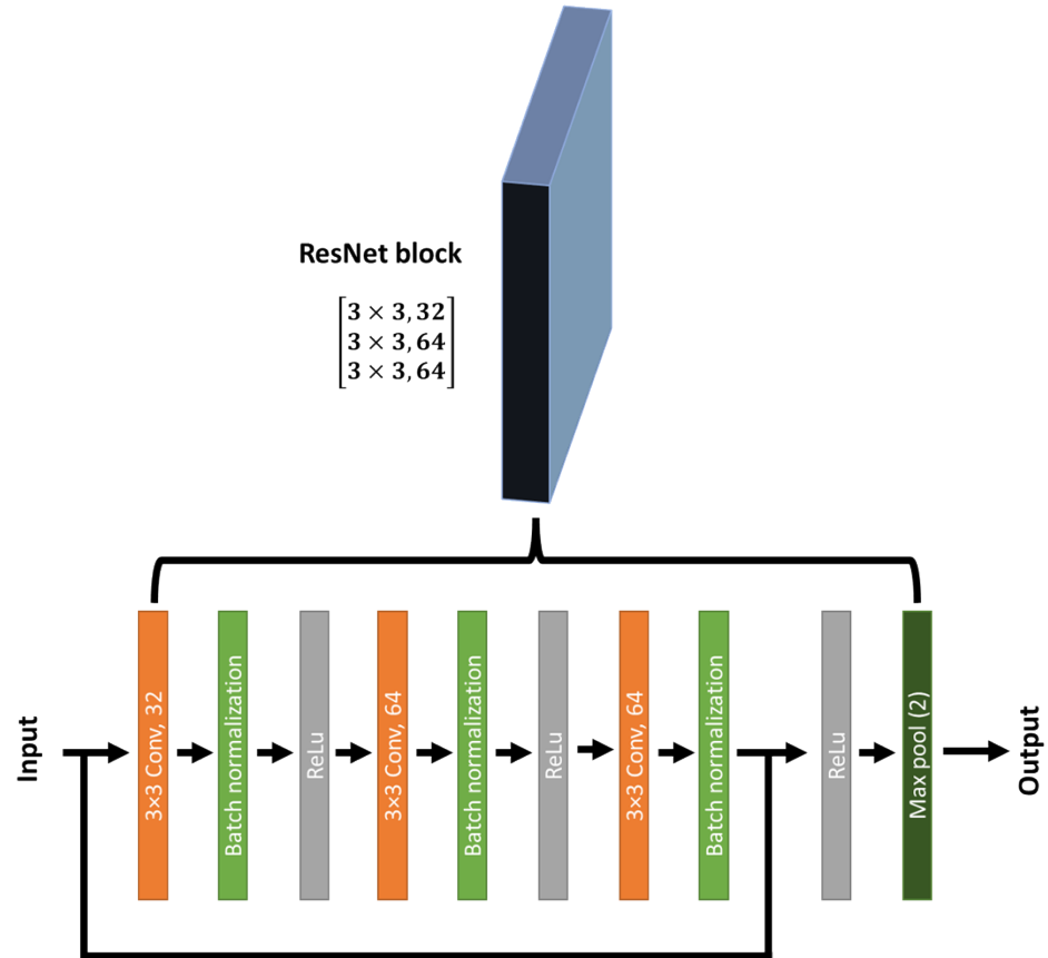
Fig. S1: Architecture of single ResNet block
